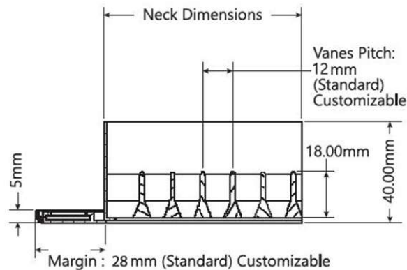
SECTION B-B
