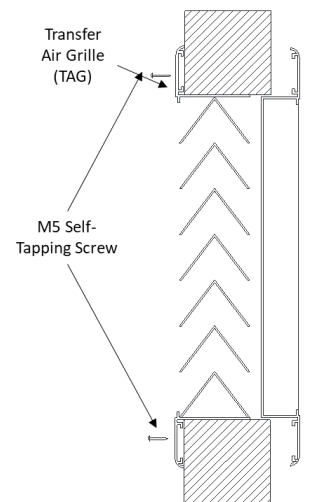
Countersunk Mounting
