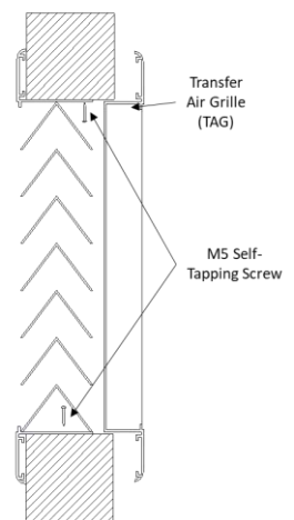
Concealed Mounting
