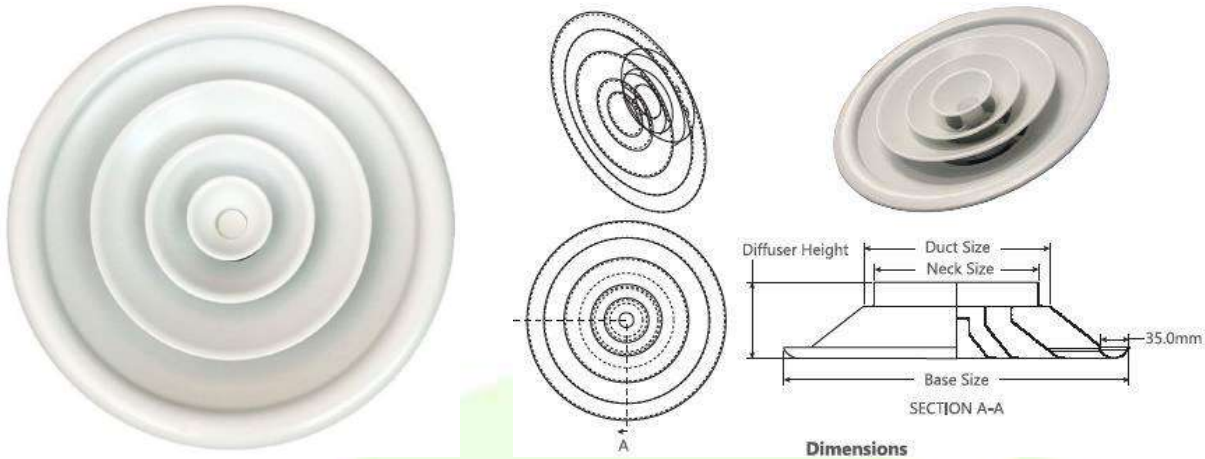
ROUND DIFFUSER
